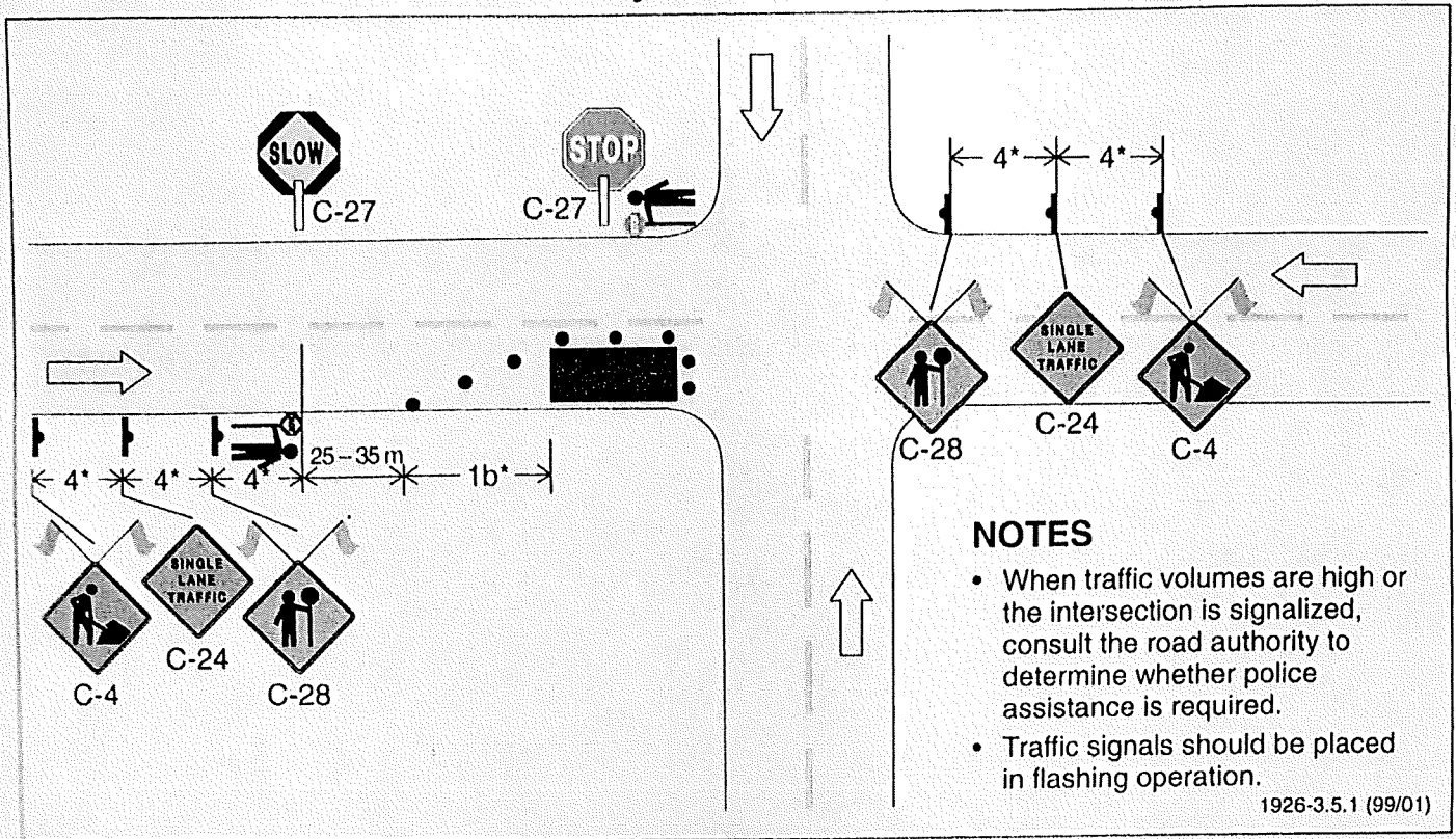
Figure 3.5.1 One Lane Closed (Near Side) - Two Lane Two-way Intersection
